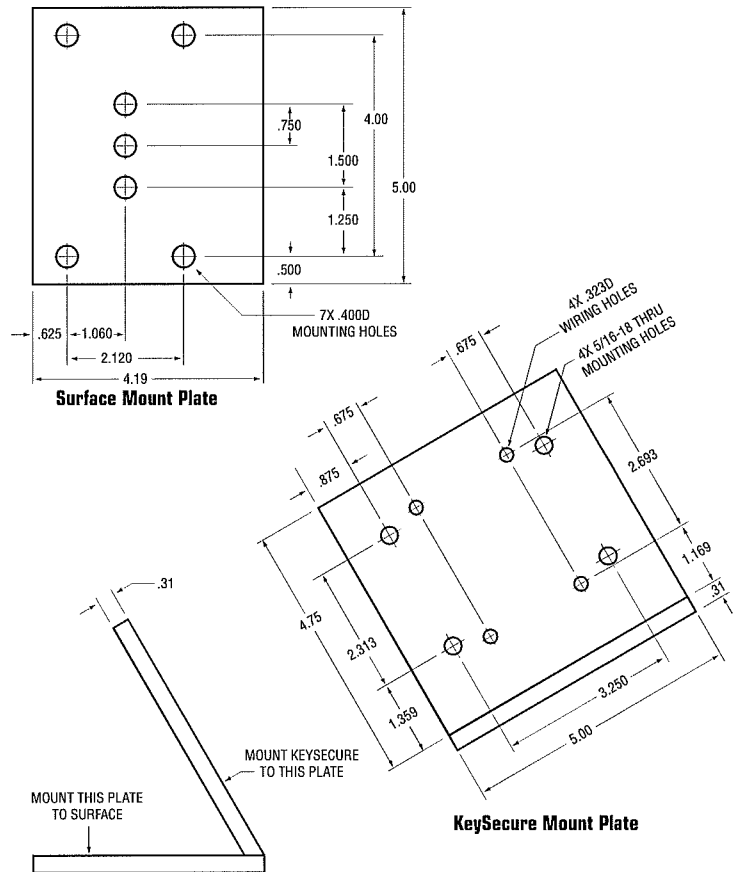
60° Bracket Mounting Holes
