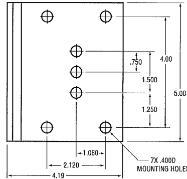
Surface Mount Plate
