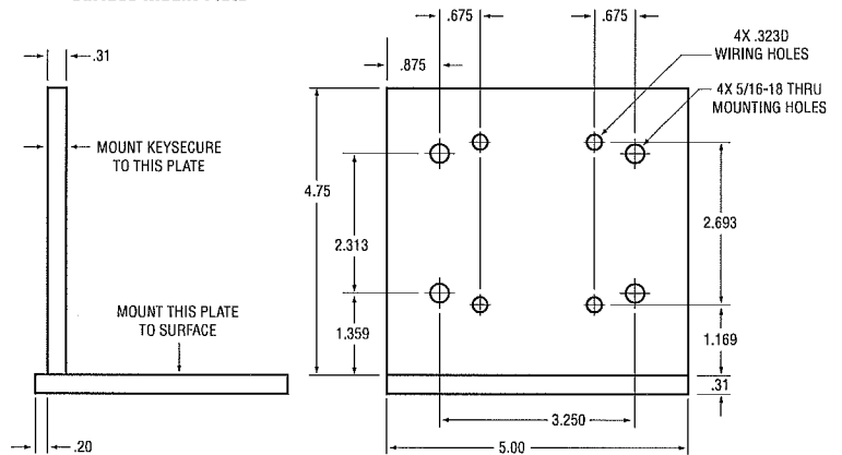
KeySecure Mount Plate
