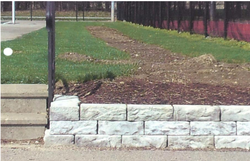
COMPLETED 480 sf Infiltration Trench with decorative stone and 660 sf 1' tall raised bioretention planter
